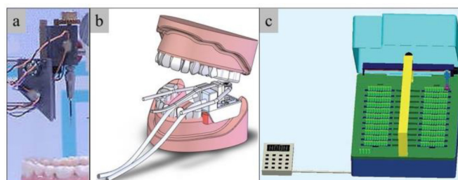
Fig. 10. Endodontic micro-robot: (a) first version micro-robot [99], (b) second version micro-robot [101], (c) model of the canal vending machine [102].
