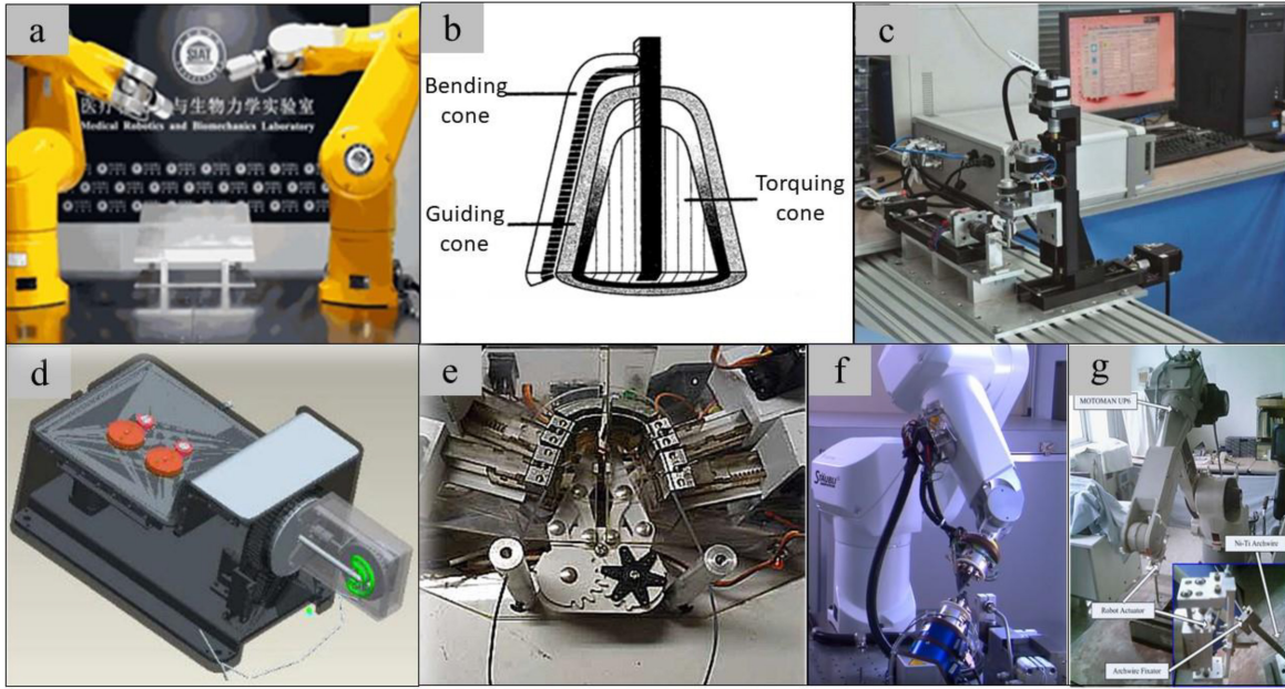
Fig. 11. Cartesian bending robots. (a) multi-arm robot [19], (b) BAS [94], (c) 5-DoF bending system [95], (d) 3-DoF bending system [96], (e) LAMDA [97], (f) SureSmile [98], (g) single-arm robot [99].
