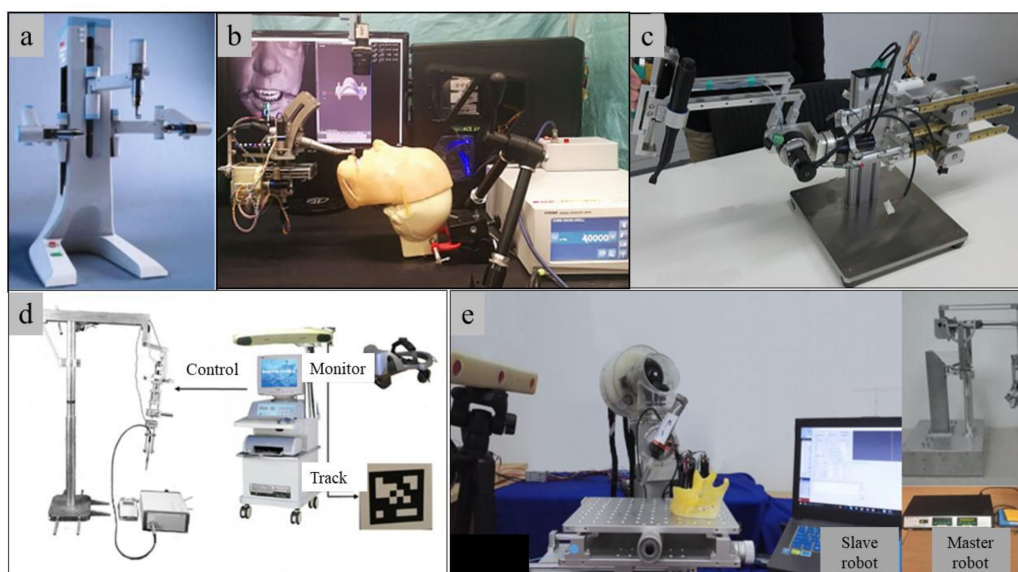
Fig. 4. Drilling robot systems for CMF surgeries: (a) three-arm robot [51], (b) remote center of motion mechanism [53], (c) master-slave surgical robot [53], (d) augmented reality-based robotic system [54], (e) master-slave surgical robot [56].
