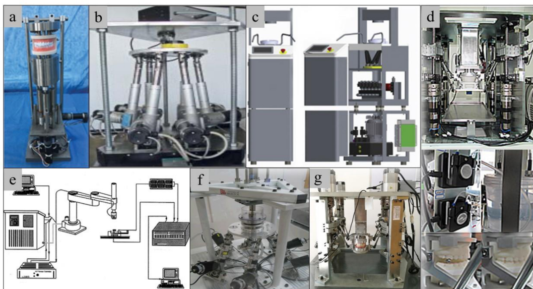
Fig. 7. Denture testing robots. (a) 5-DoF IDR [78], (b) Conserva et al. [79], (c) Tahir et al. [81], (d) DUT-2 [83], (e) measurement system for mastication force [86], (f) Waseda-Yamanashi [87], (g) redundantly actuated parallel manipulator (RAPM) prototype [88].
