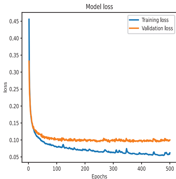
FIGURE 6 Mean training and validation loss of five-folds.
